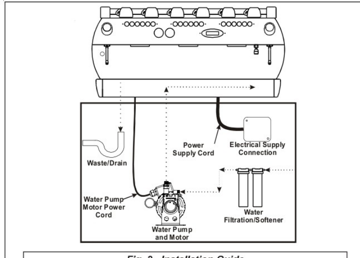
Fig. 2 - Installation Guide
